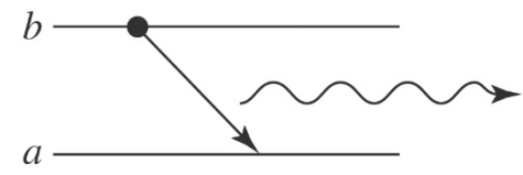
(c) Spontaneous emission
