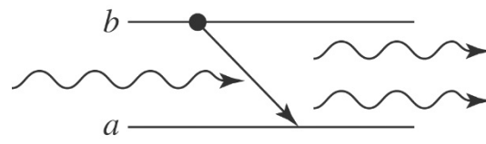
(b) Stimulated emission
